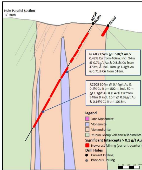
Figure 11. Schematic Cross Section RC603.
