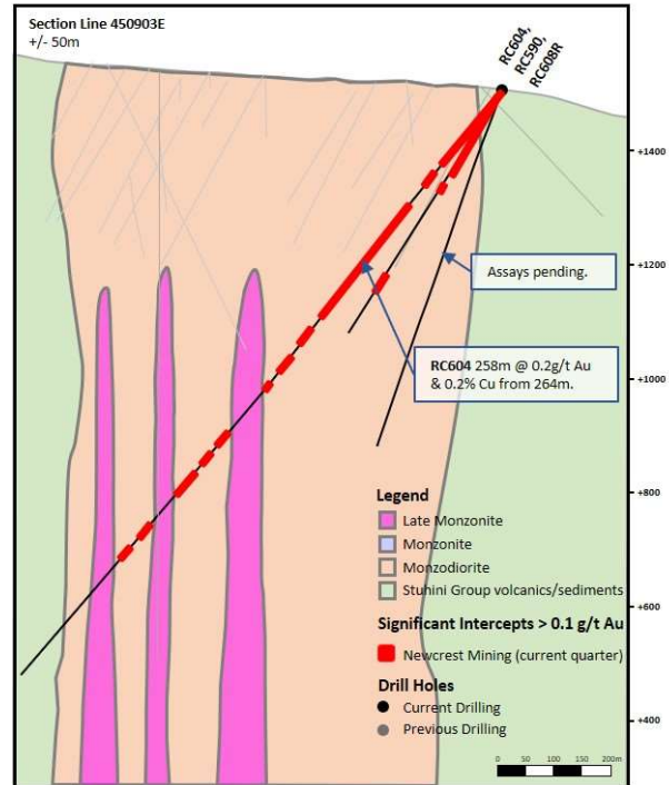
Figure 12. Schematic Cross Section RC604.
