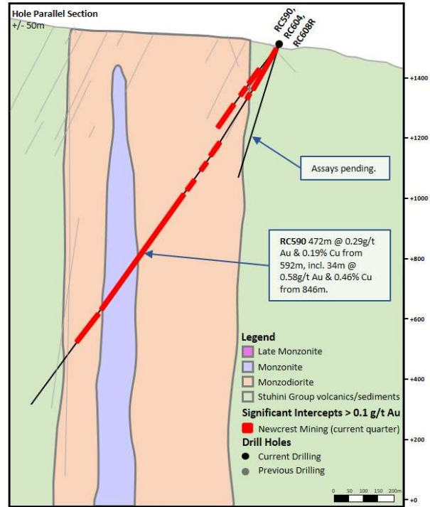
Figure 10. Schematic Cross Section RC590.
