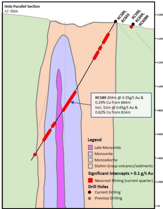
Figure 9. Schematic Cross Section RC589.
