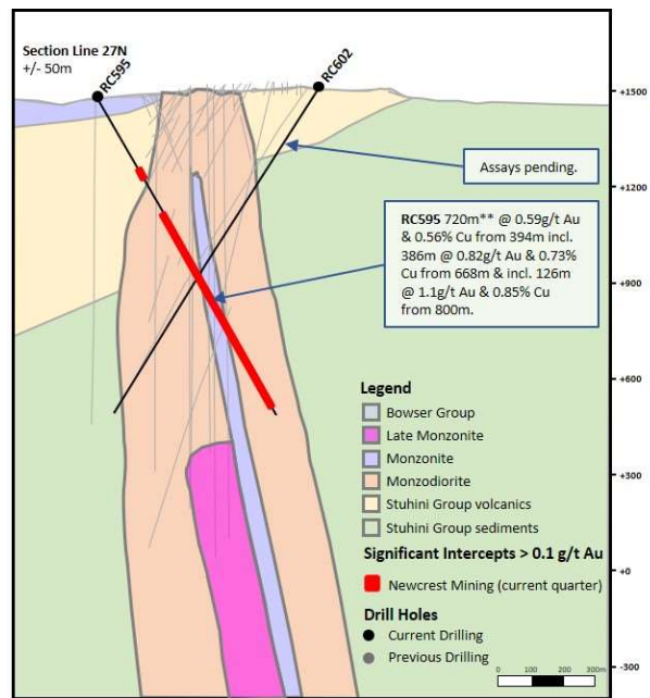
Figure 8. Schematic Cross Section RC595.
