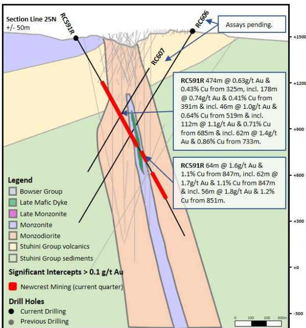
Figure 7. Schematic Cross Section RC591R.
